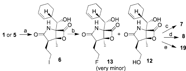
Scheme 3. Synthesis of Tosyl ( 7 ), Mesyl ( 8 ) and Dansyl ( 19 ) Derivatives a
