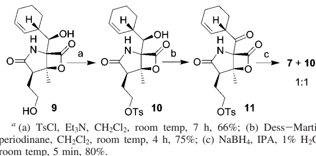
Scheme 3. Synthesis of Tosyl ( 7 ), Mesyl ( 8 ) and Dansyl ( 19 ) Derivatives a
